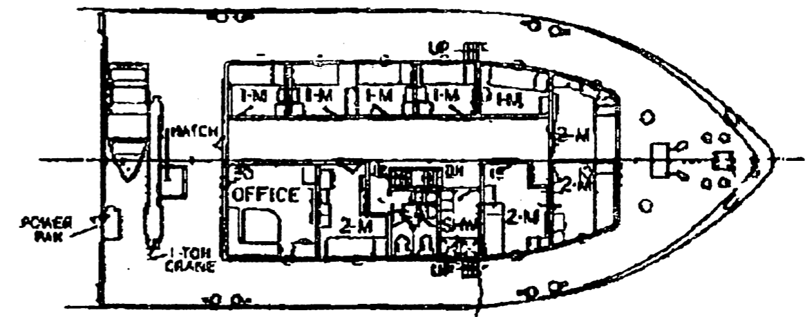
FOC'SLE DECK
