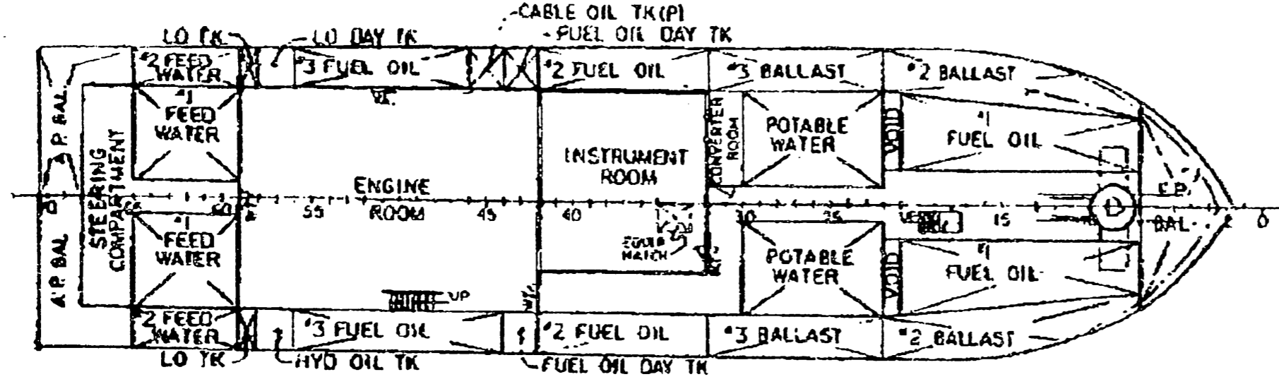
HOLD PLAN
