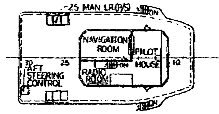
PILOT HOUSE
