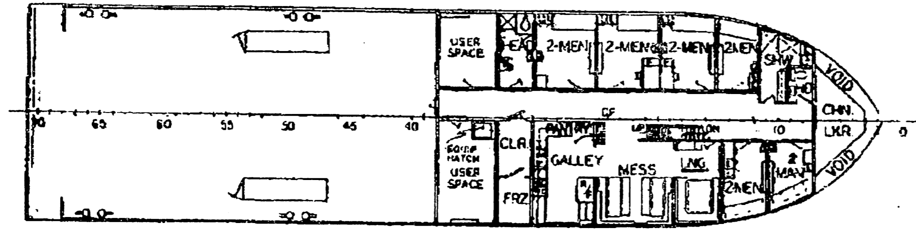
MAIN DECK
