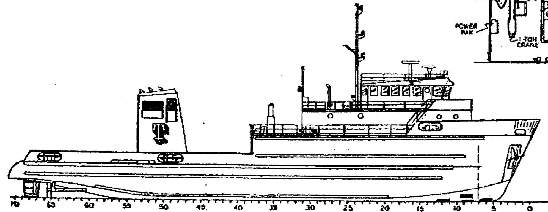
OUTBOARD PROFILE
